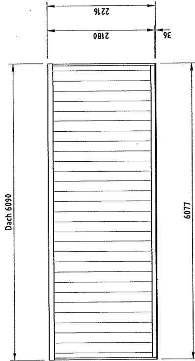
TURWAND
